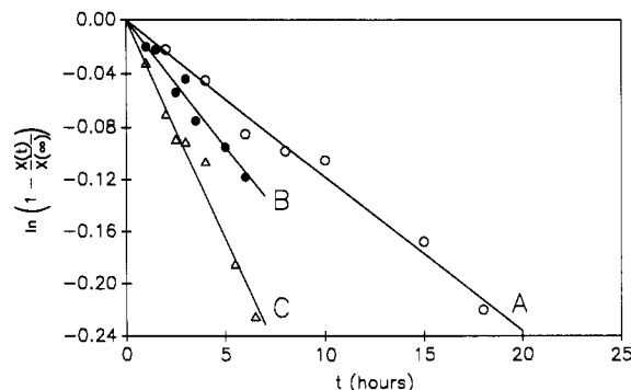
FIGURE 1: [^3\text{H}] POPC transfer from POPC SUV for 0.01 mM donors at 30^\circ\text{C} . Acceptor concentrations are (A) 0.5; (B) 10.0, and (C) 20.0 mM. Points represent averages obtained from triplicate experiments consisting of at least eight data points.
